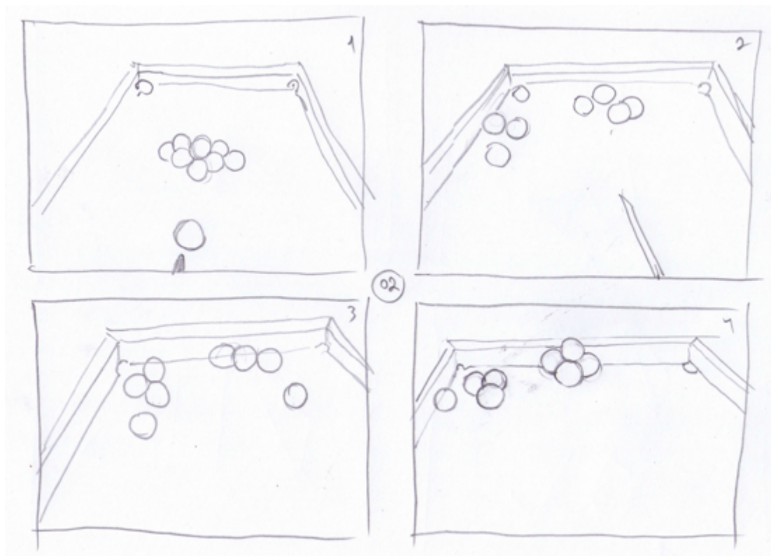
Figure 6.2 Billiard game
