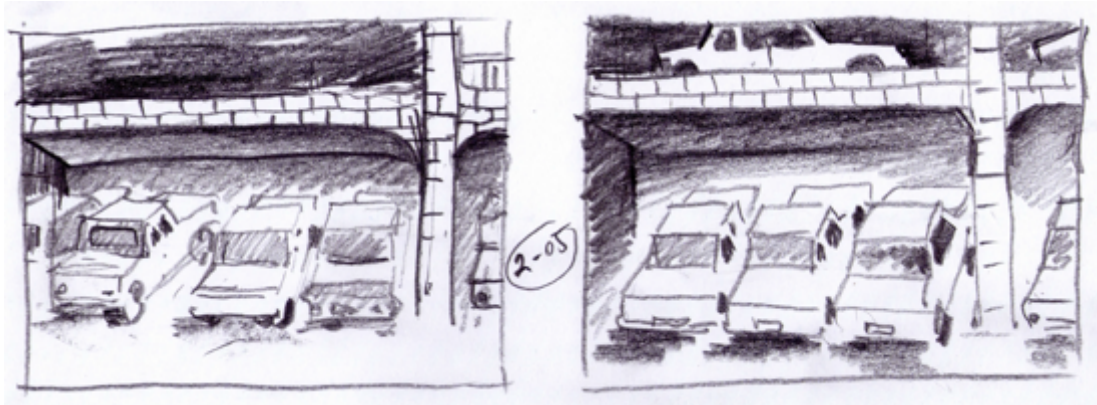
Figure 6.6 Parking lot
