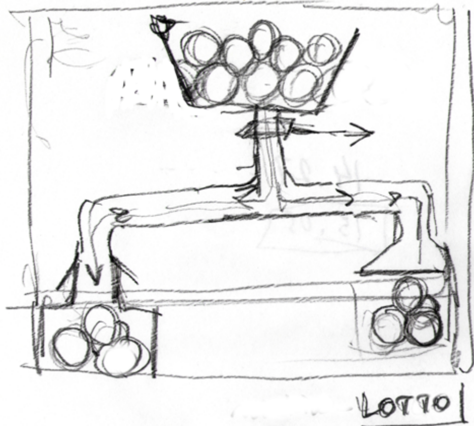
Figure 6.1 Lottery machine
